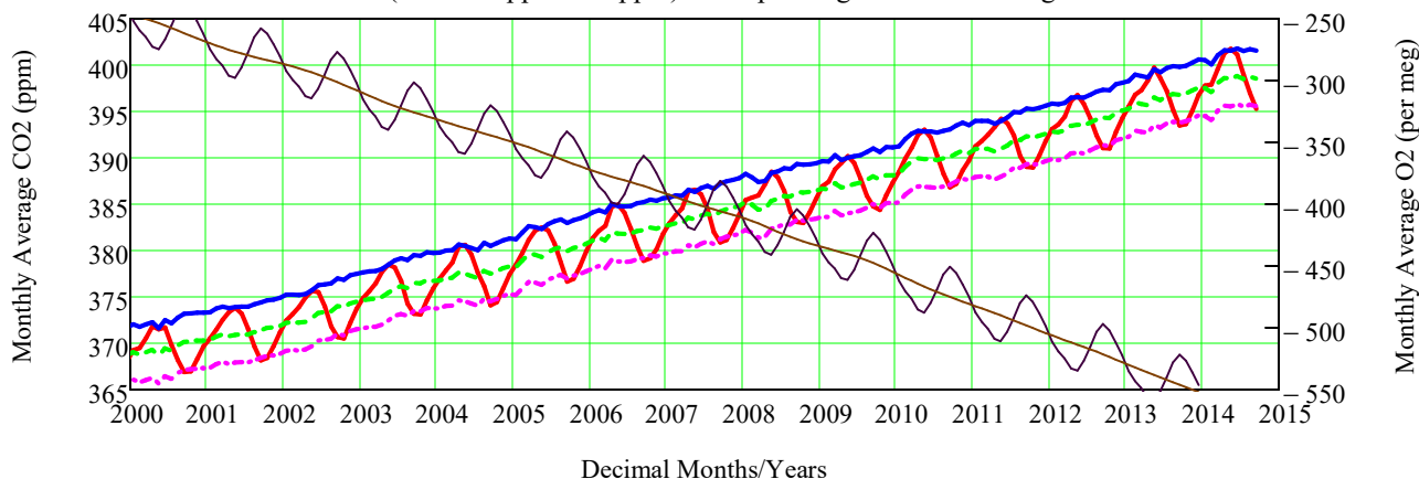
2b. Mauna Loa CO2 (Seasonal ppm +/- 3 ppm) & O2 per meg: Seasonal Swing about Trend Line
