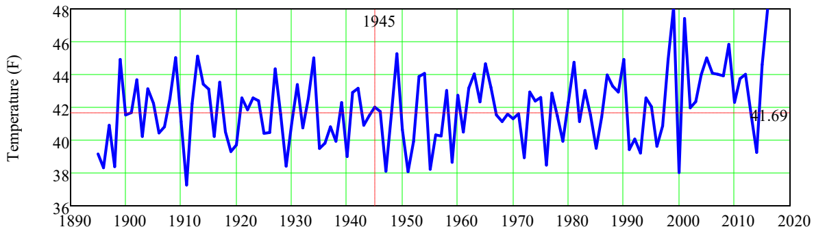
12. NOAA US Annual Mean Temperature 1895 to 2016 Mean Temp 41.69 F
