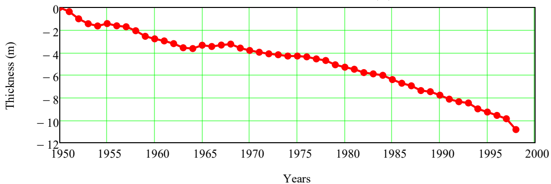
2. Glacier Cumulative Mass Balance, Thickness (m) - 1950 to 2000
