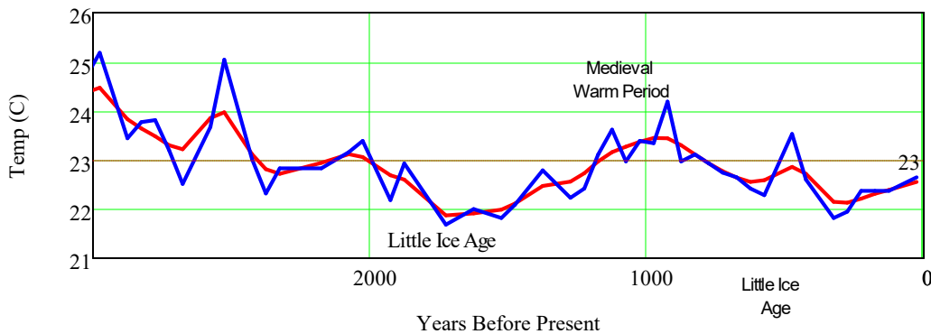
4. The Little Ice Age and Medieval Warm Period. Sargasso Sea Surface Temperature
