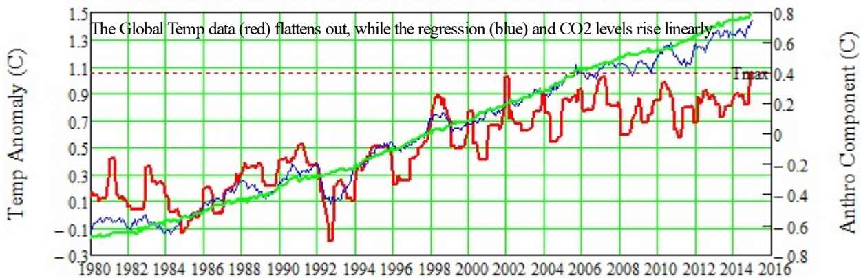
Temp Data (Red), MultiVariate Regression (Blue), b4*z4 (Green)
