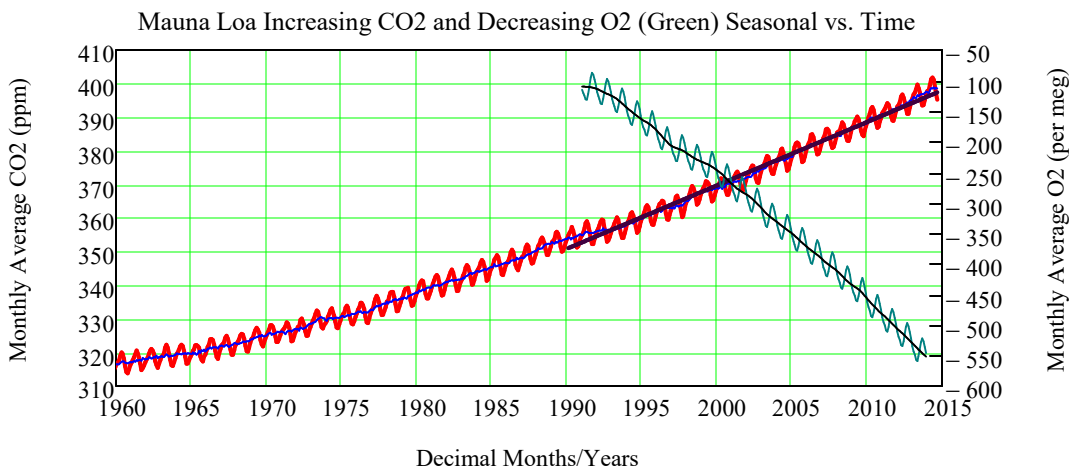
2b. Mauna Loa CO2 (Seasonal ppm +/- 3 ppm) & O2 per meg: Seasonal Swing about Trend Line
