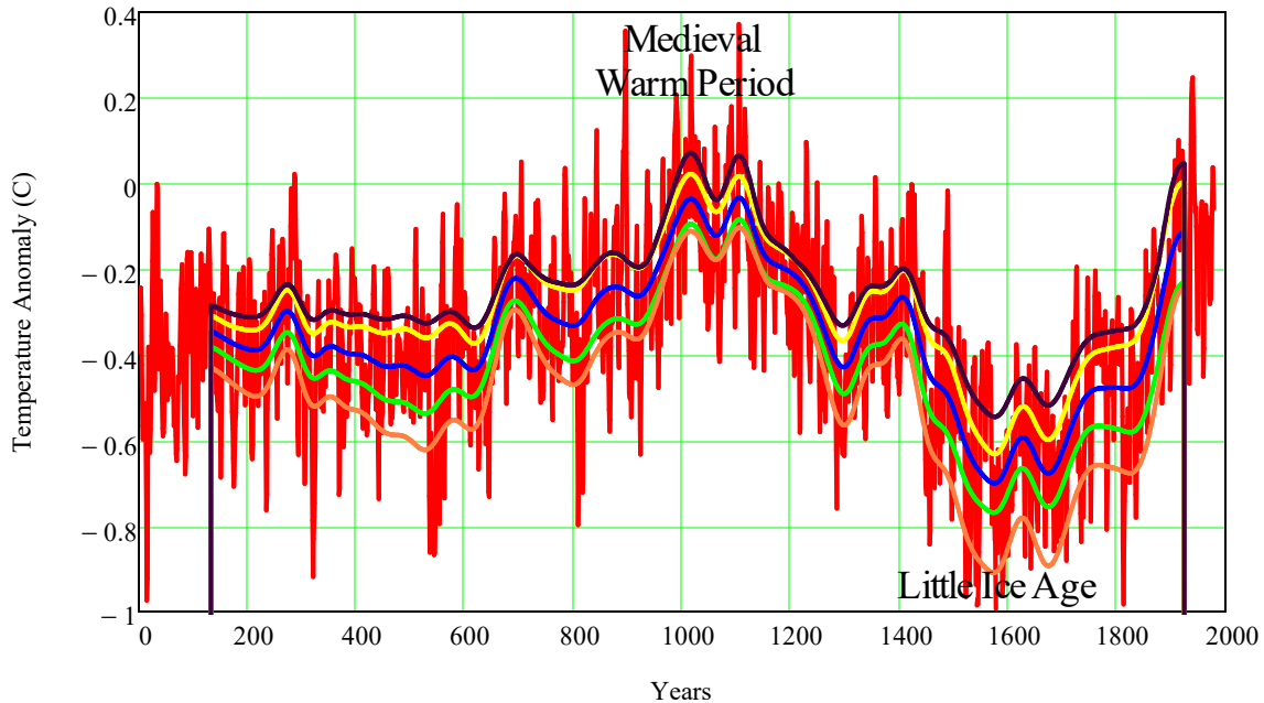
8. Multi-Proxy Reconstruction North Hemisphere Temperature Anomaly
