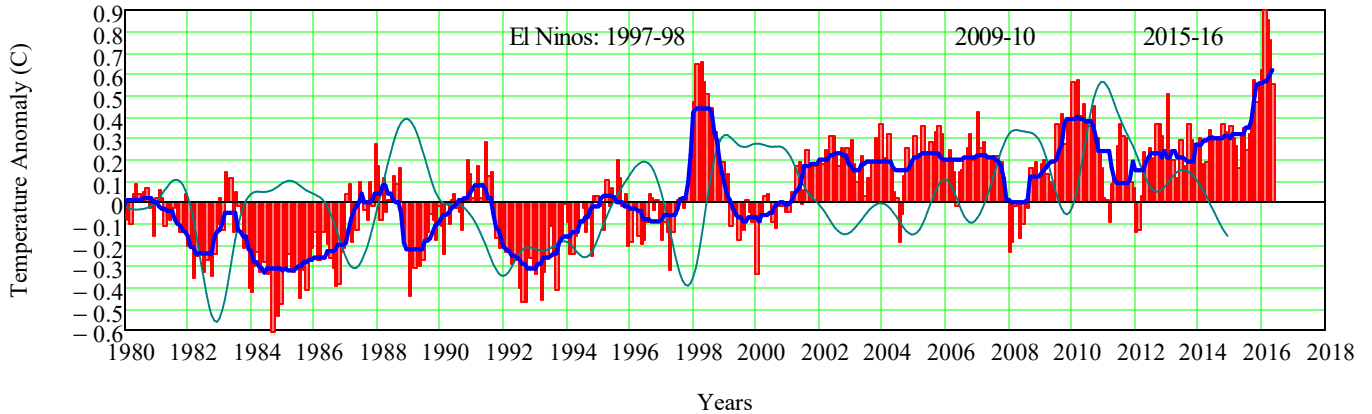
7A. UAH Satellite Global Temp Anomaly, 13 Month Avg (Blue), and Southern Oscillation Index, SOI - (Green)
